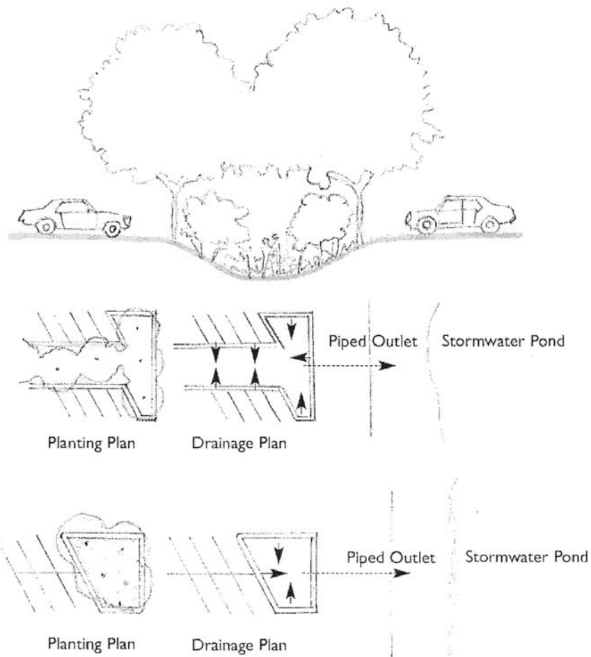
Figure 7.28. Parking Lot Stormwater Retrofit Schematics
