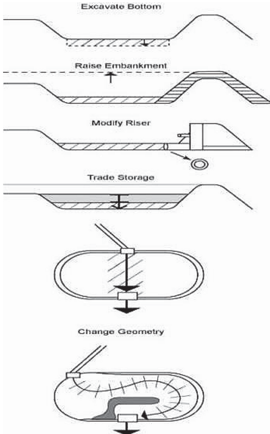
Figure 7.10. Some Modifications That Can Be Made to Existing Detention Ponds. Source: CWP 2007
