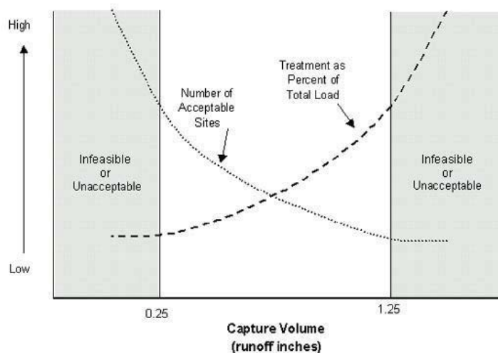
Figure 7.6. Optimization Point for Retrofit Treatment
