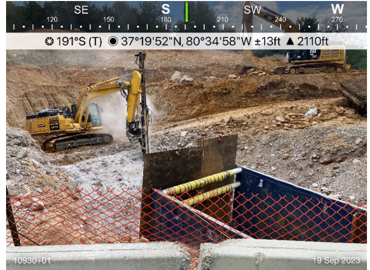
Figure 2: Bore site for S-Y2 &S-Y3 at Sta10930+01, ECD's are in place.
